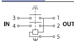
TRACON SSTM-015
