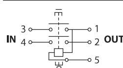
TRACON SSTM-035
